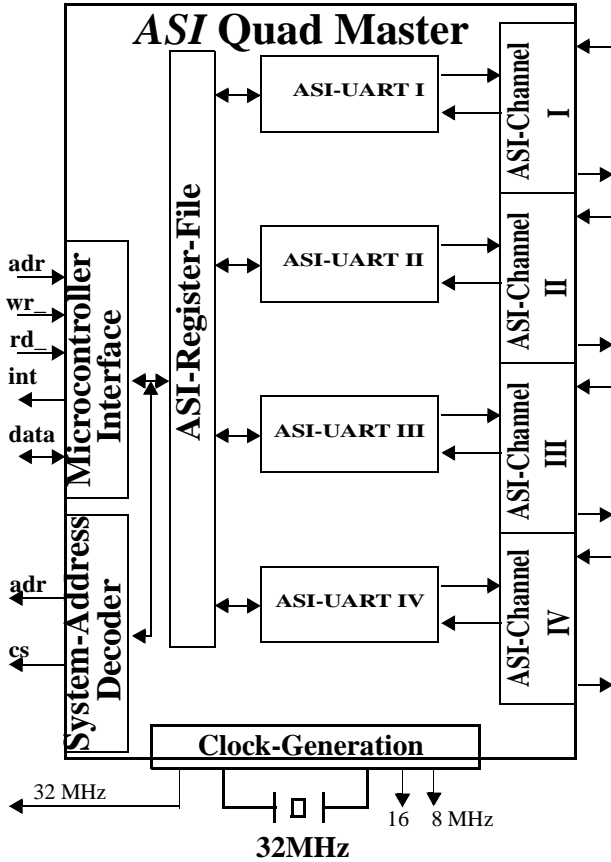
Figure 6. Architecture of the ASI Quad Master
