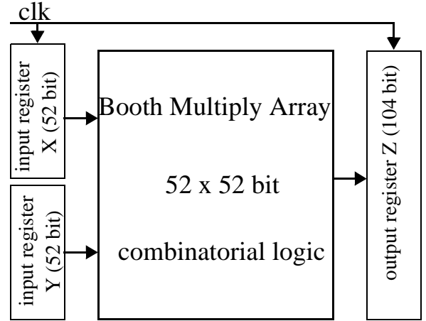
Figure 7. Multiply-Core of the FPU
