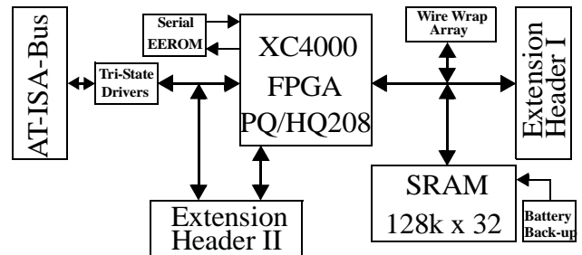
Figure 4. Architecture of SPYDER-ASIC-X1
