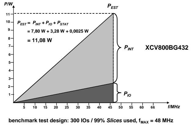
Figure 5. Power consumption on Virtex FPGAs
